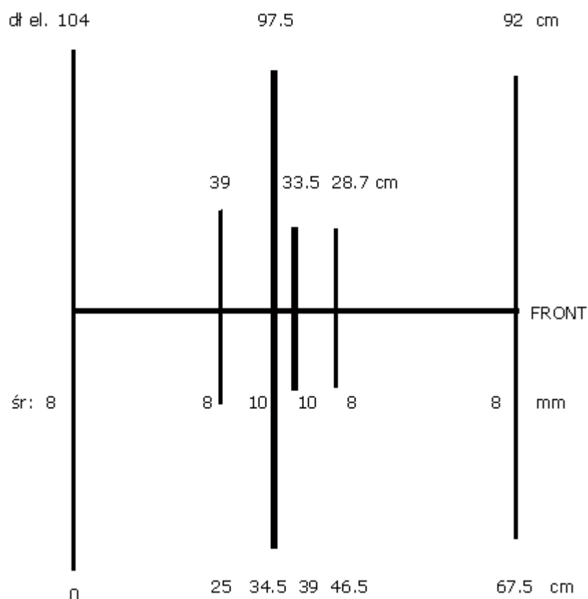
ANT DUAL YAGI 3 el. 2m/70cm SP4IZK
